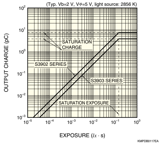
Figure 6 Output charge vs. exposure
