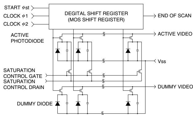
Figure 1 Equivalent circuit
